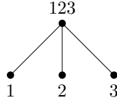
Fig. 3. A separative poset which does not satisfy (\ddagger^f) .
