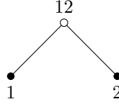
Fig. 2. A structure from \mathbf{T} + (\dagger) which is not an element of \mathbf{T} + (\dagger^f)
